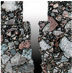
Routed Cracks increase crack seal longevity.
